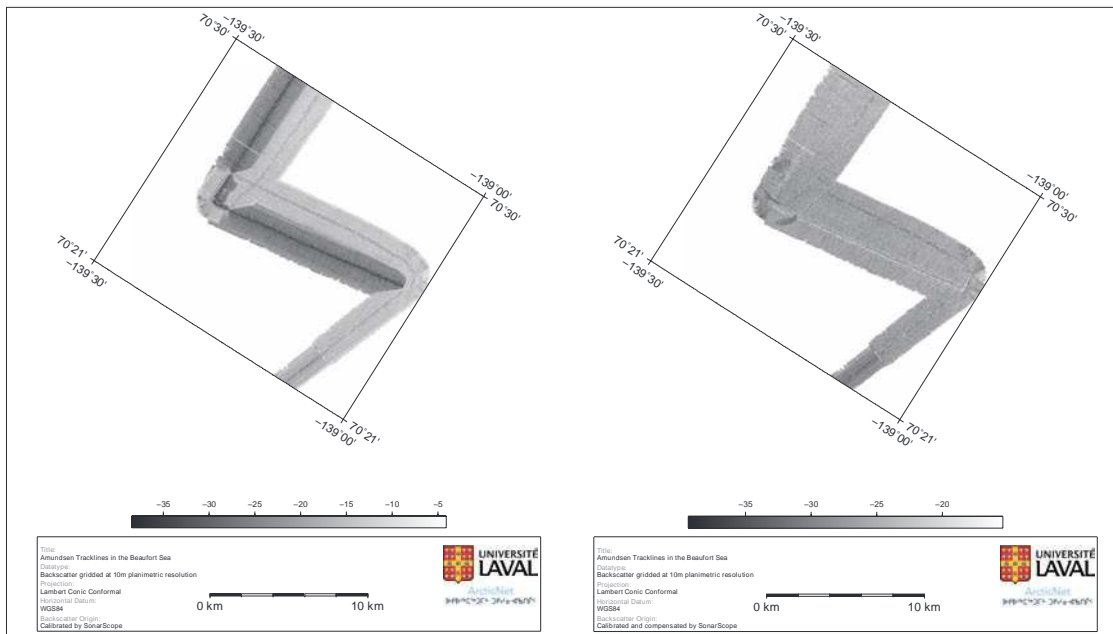
Fig. 7: Angular compensated BS mosaic following the transmission sector pattern calibration (a, left) and following a statistical compensation to remove the remaining 0 dB interline bias (b, right)
