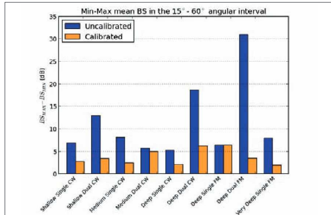
Fig. 6: Precision of the angular compensated mean BS in the 15 to 60 degrees angular interval for all operational Transmission Modes of the EM300 of CCGS «Amundsen»
