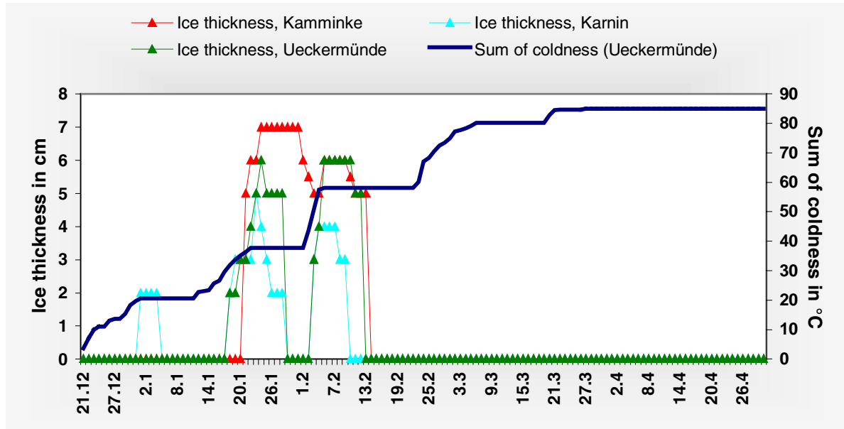
Figure 7.4. Accumulated sum of coldness and measured ice thickness in the Szczecin Lagoon in the winter of 2000/01
